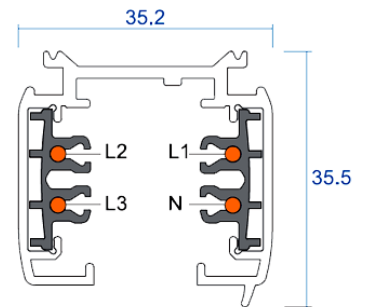
Rail 3 allumages
