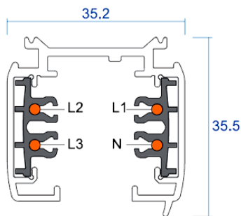
Rail 3 allumages
